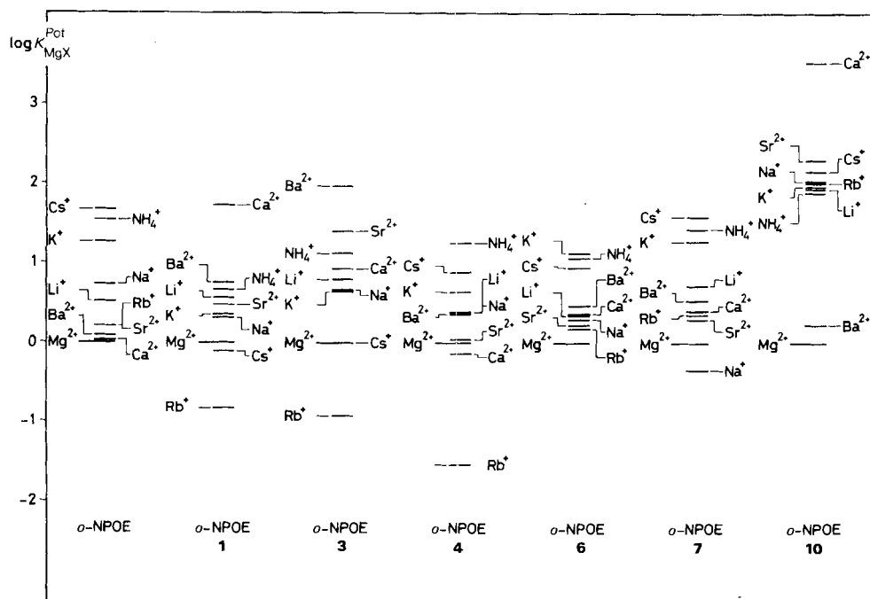
Fig. 1. Selectivity factors, \log K_{MgX}^{Pot} , for solvent polymeric membranes with o -nitrophenyl octyl ether ( o -NPOE) as membrane solvent. Ligand-free membranes (column 1) are compared with membranes containing different ligands (separate solution method, 0.1M solutions of the chlorides, 20–22°).
